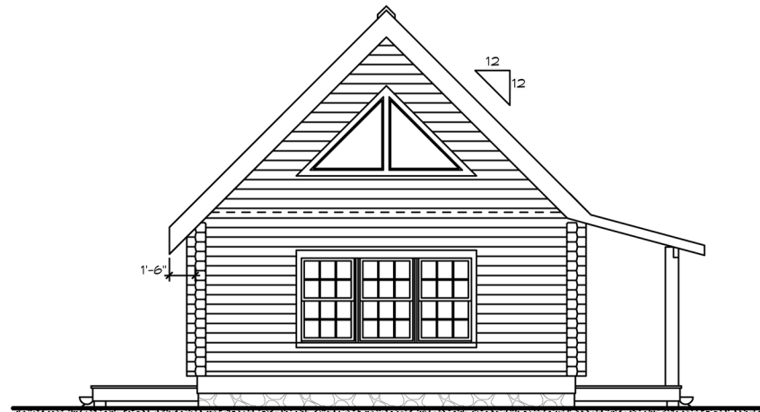
LEFT ELEVATION
